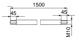
ES-G2083E Barra tirante lunghezza standard 1500 mm. Connecting rod standard length 1500 mm. Zugstange Lager?nge 1500 mm.
